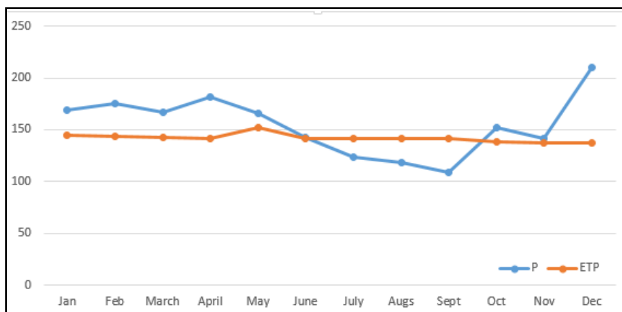
Fig. 2. Water balance East Kalimantan province
